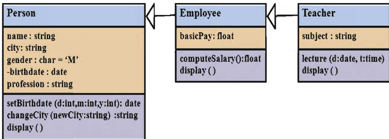
Figure 6.9 : Example of multilevel inheritance
