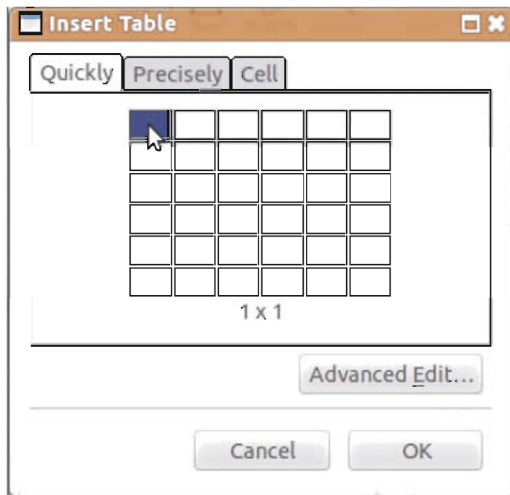
Figure 3.3: Insert 1×1 Table
